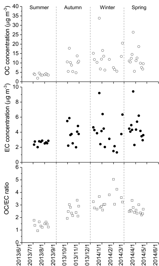
Figure 1. Temporal variations of OC and EC mass concentrations as well as OC/EC ratio of PM 1 samples in Beijing.
