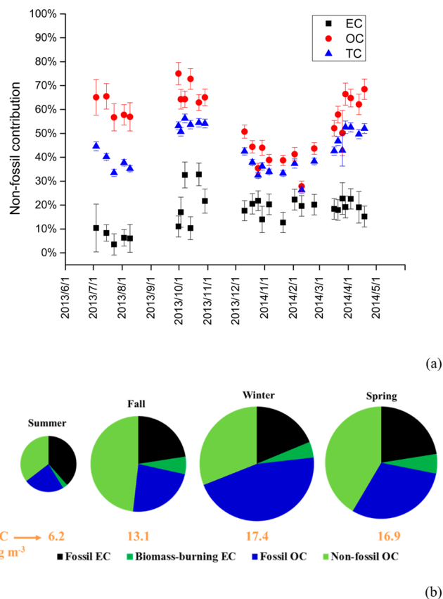
Figure 2. (a) Temporal variations of nonfossil contribution to OC, EC, and TC and (b) average source apportionment results of TC in each season of PM 1 samples in Beijing. The numbers below the pie chart represent the average TC concentrations for each season.
