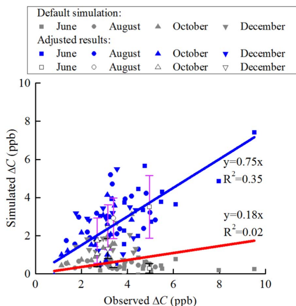
Fig. 6. Correlations between the observed and scaled daily N_2O mixing ratio enhancement ( \Delta C ) at the KCMP tower at 185 m. Error bars represent one standard deviation of default simulation (black) and adjusted results (blue). (For interpretation of the references to colour in this figure legend, the reader is referred to the web version of this article.)
