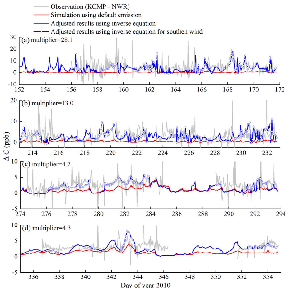
Fig. 5. Comparison of \text{N}_2\text{O} mixing ratio enhancement ( \Delta C ) between observation (grey line), default model simulation (red line), and the scaled model simulation (blue line) for the height of 185 m at the KCMP tower site. Periods with south wind (wind direction: 90^\circ\text{--}270^\circ ) are marked by dots. (For interpretation of the references to colour in this figure legend, the reader is referred to the web version of this article.)
