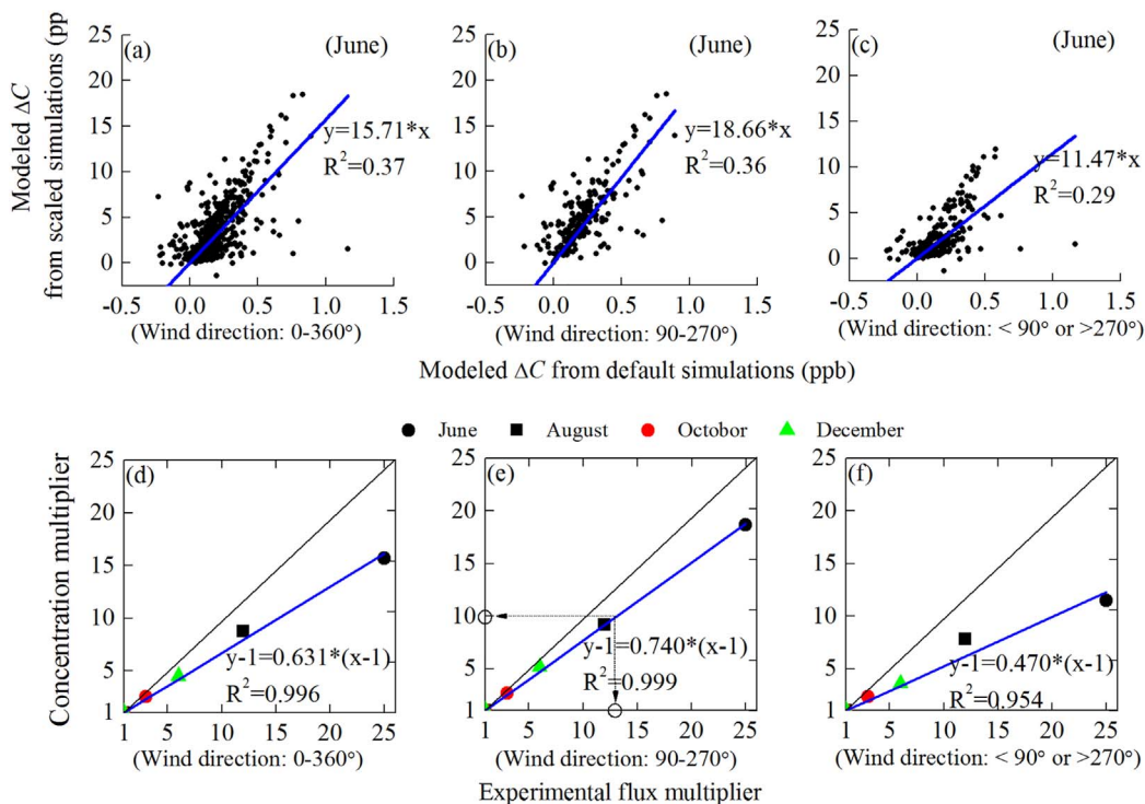
Fig. 4. Relationships for different model runs between concentration multiplier and experimental flux multiplier. The modeled N_2O mixing ratio enhancement \Delta C was obtained from default and scaled simulations for 185 m at the KCMP tower. The scale simulation shown in panels a–c uses a multiplier of 25.0. The regression slope in panels a–c is represented by the black circle in panels d–f. The hollow dots and dot lines in sub-figure (e) show how the emission flux multiplier M_F (the dot on x axis) is induced via the concentration multiplier M_C (the dot on y axis) for October 1–20.
