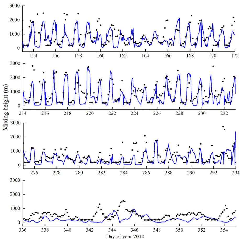
Fig. 3. Simulated mixing height and the NCEP-NARR data (dots) for the four simulation periods.
