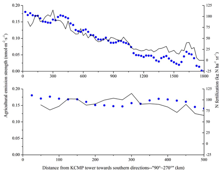
Fig. 8. Agricultural \text{N}_2\text{O} emission strength and N fertilization rate as functions of distance from the KCMP tower in the south wind sector ( 90^\circ\text{--}270^\circ ).
