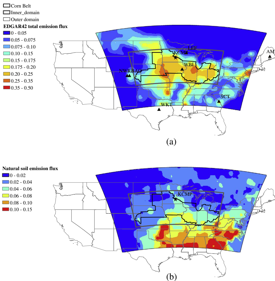
Fig. 1. Locations of the \text{N}_2\text{O} monitoring sites, scope of the Corn Belt, modeling domains, and the prior \text{N}_2\text{O} emission flux in \text{nmol m}^{-2} \text{s}^{-1} . (a) EDGAR42 emission flux, (b) natural soil emission flux. KCMP – Minnesota; NWR – Niwot Ridge, Colorado; AMT – Argyle, Maine; BAO – Boulder Atmospheric Observatory, Colorado; LEE – Park Falls, Wisconsin; SCT – Beech Island, South Carolina; WBI – West Branch, Iowa; WKT – Moody, Texas.
