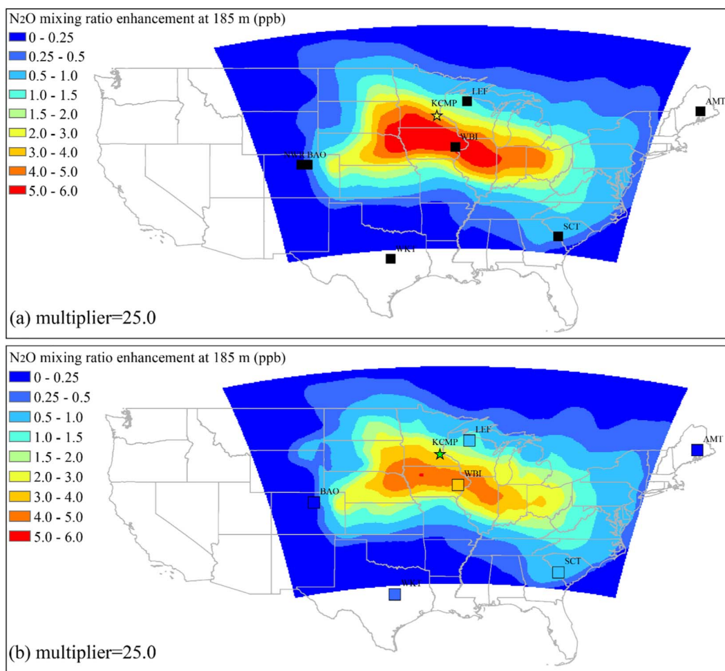
Fig. 7. Spatial characteristics of the mean modeled N 2 O mixing ratio enhancement during June 1–20: (a) modeled results for all hours; (b) modeled results for UTC hours 19 and 20 only.
